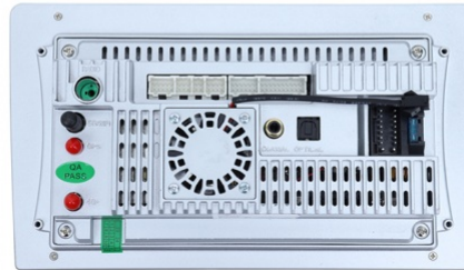
Head Unit Back Side
